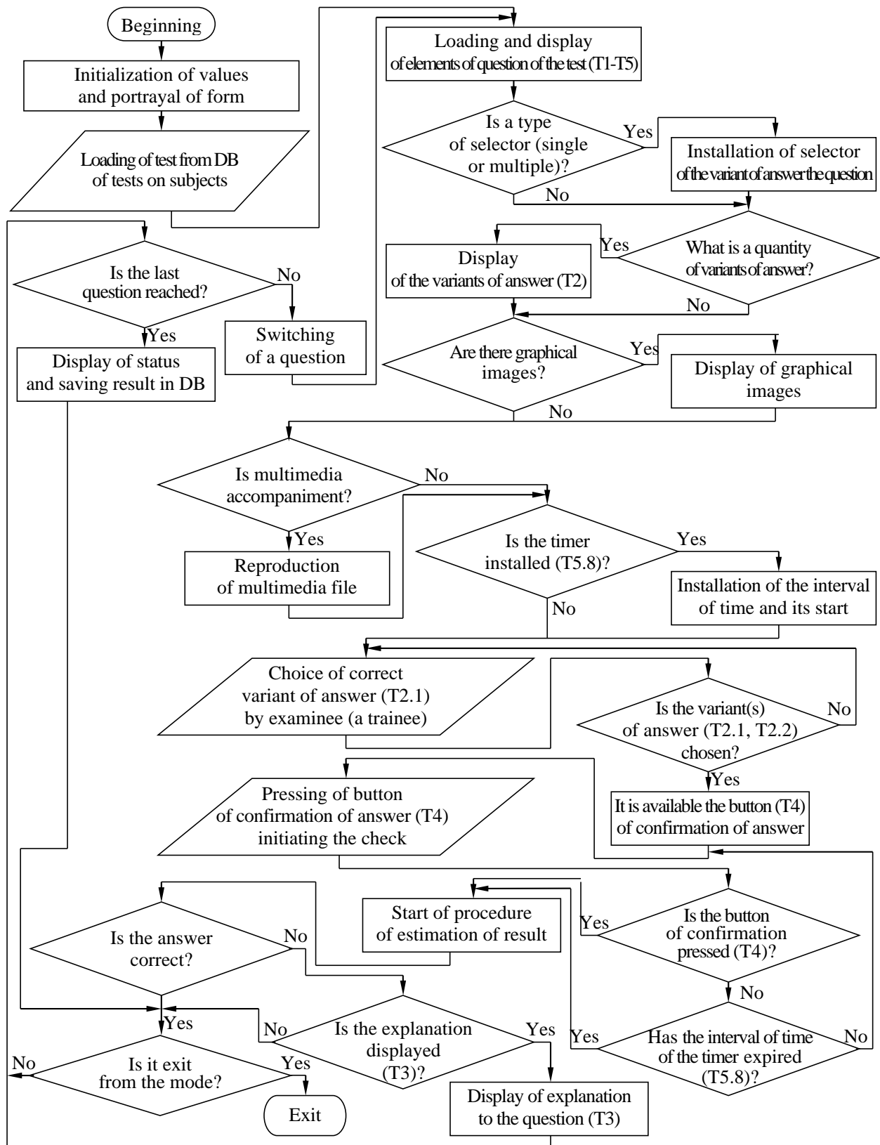
Pic. 6.15. The algorithm of support of functioning of the mode of diagnostics for the estimation of the level of residual knowledge of a trainee
