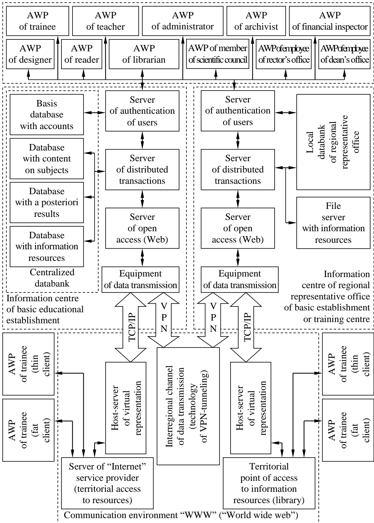
PIC. 2.3. The standard scheme of interaction of the information centre of educational establishment and the automated workplaces of the subjects of training. The territorially distributed AWP of the subjects of IEE of ART interact with the certain information centre of EEs by means of use the network "Internet".
