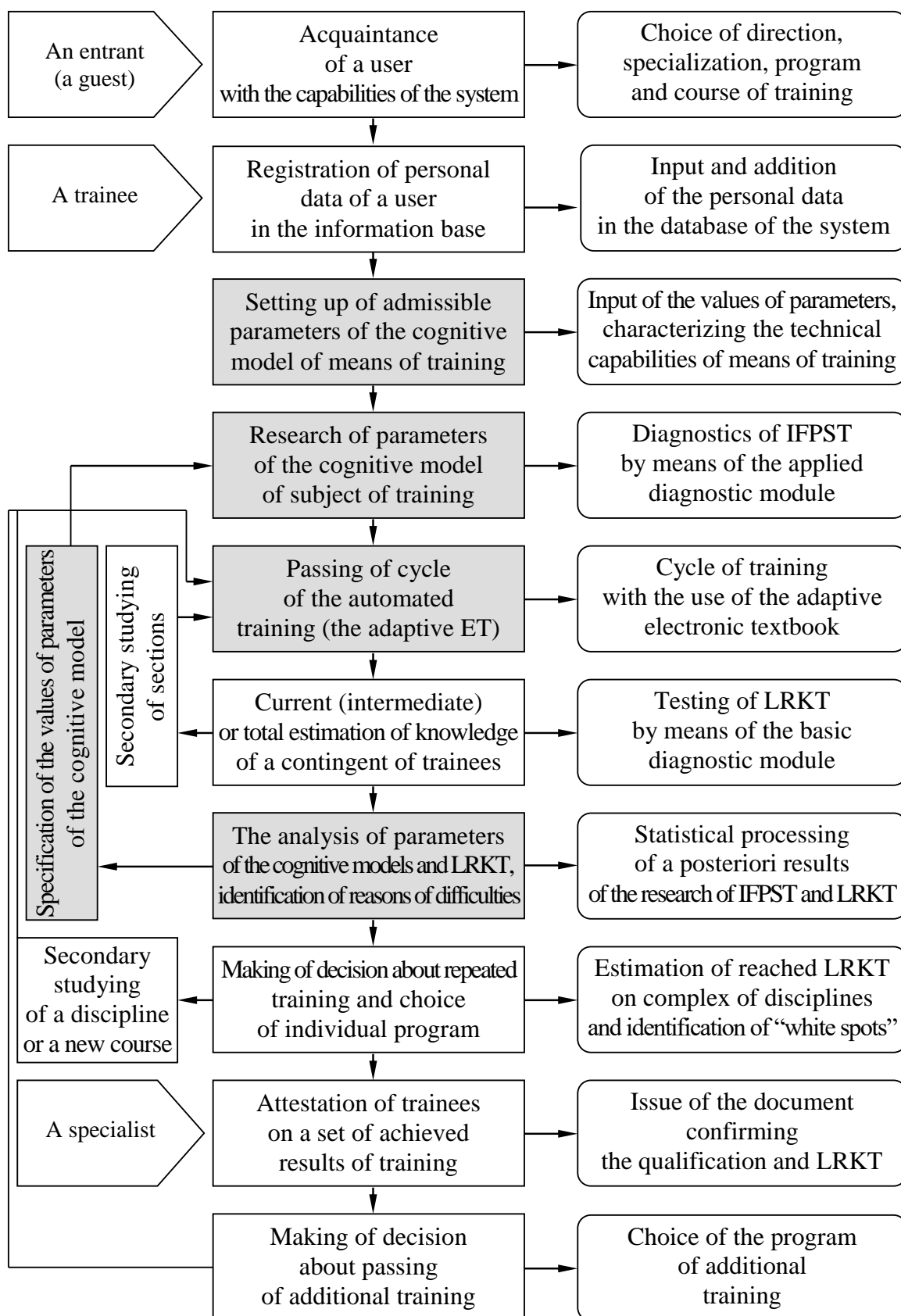
Pic. 7.1. The scheme, reflecting the sequence of actions for the support of researches of the cycle of the adaptive automated training
