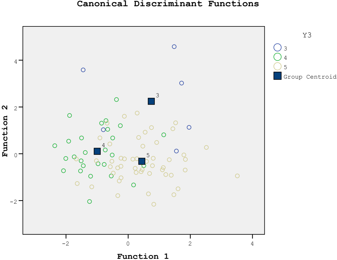
Pic. 7.13. The chart of distribution (geometrical arrangement) of the centroids of classes in the space of the canonical discriminant functions
