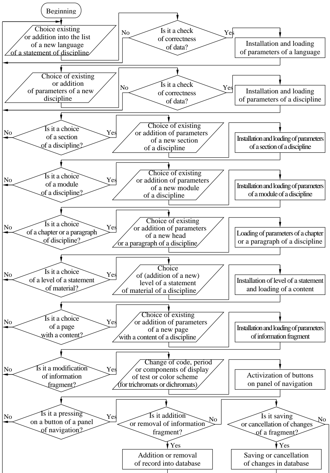
Pic. 6.8. The algorithm of formation of the database (knowledgebase) with filling in subjects of studying of the adaptive means of training (electronic textbook)
