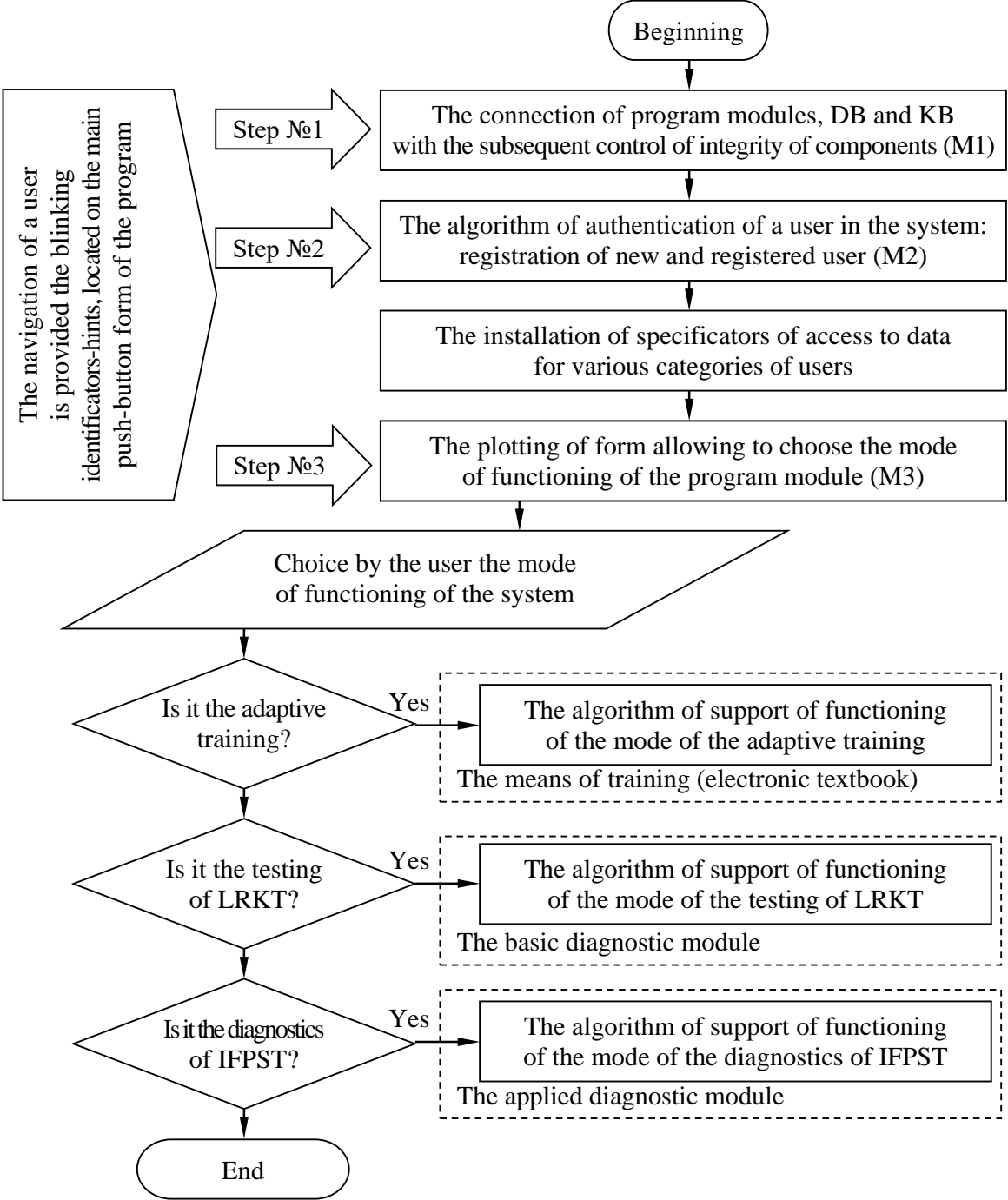
Pic. 6.2. The algorithm of switching of the modes of functioning of the program complex
